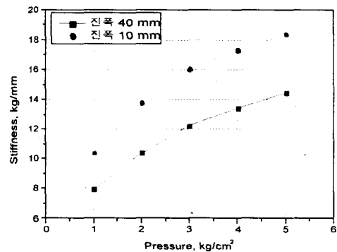
Fig. 19 Static and Dynamic Stiffness of Horizontal Direction
