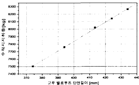
Fig. 10 Vertical Load for Various Sectional Length
