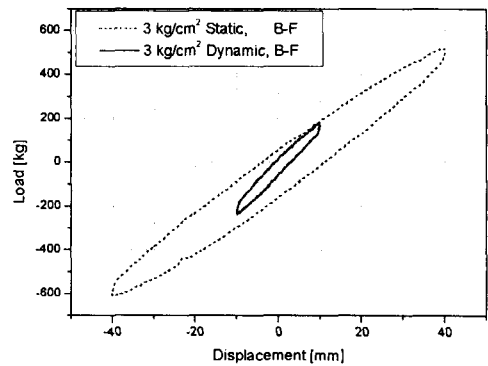
Fig. 18 Load-Displacement Curves of Horizontal Direction
