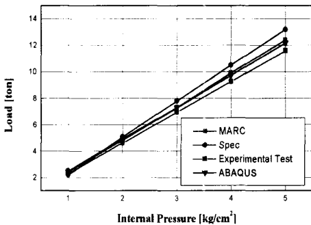
Fig. 7 Diagram of Pressure-Vertical Load
