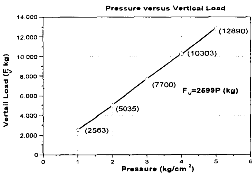
Fig. 16 Vertical Load vs. Pressure
