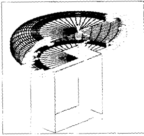
Fig. 3 3D Finite Element Model
