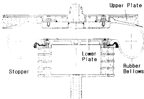
Fig. 1 Bellows Type Air Spring
