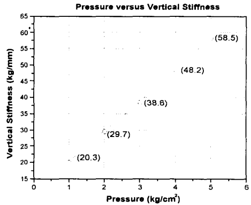
Fig. 17 Vertical Stiffness vs. Pressure
