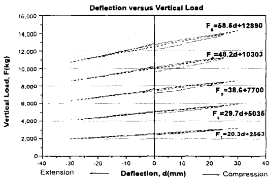
Fig. 15 Hystereses Curves for Vertical Tests
