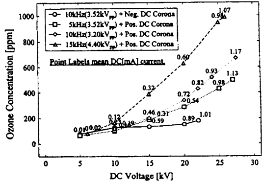
Fig. 4. Effect of superposition of two discharges on ozone generation (10kHz, 534ppm, 2 l /min)
