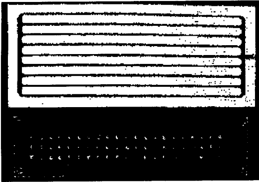
Fig. 2. Photograph of surface discharge unit(upper) and corona discharge unit(lower)
