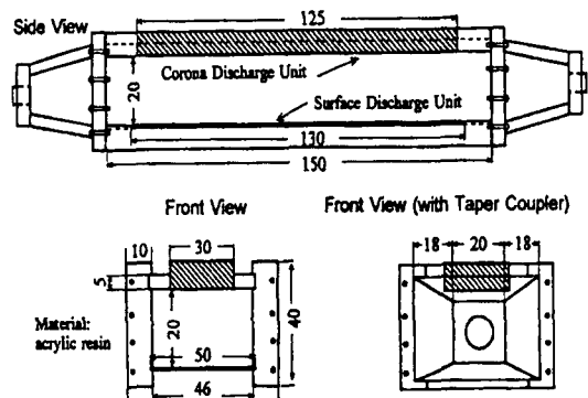
Fig. 1. Structure of plasma reactor combined with surface and corona discharge. [unit:mm]
