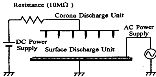
Fig. 3 Conceptual electric circuit of the experiment system
