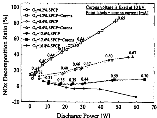
Fig. 7. Effect of superposition of two discharges on NO decomposition(3) (534ppm, 2 l/min)
