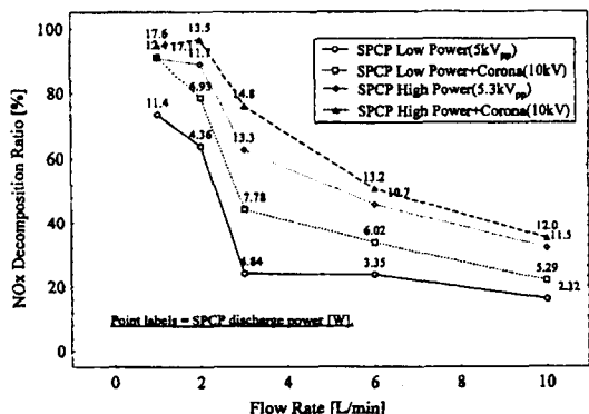
Fig. 6. Effect of superposition of two discharges on NO decomposition(2) ( N_2 balance, 534ppm)
