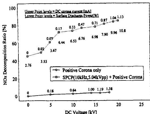
Fig. 5. Effect of superposition of two discharges on NO decomposition(1) ( N_2 balance, 534ppm, 2 l/min)
