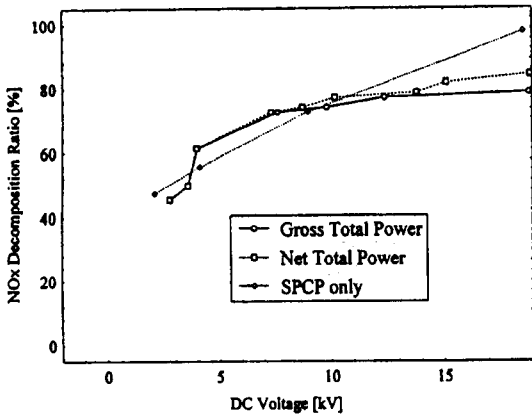
Fig. 8. Range in which energy efficiency of superposing reactor surpasses that of normal reactor
