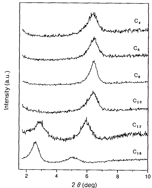
Figure 4. X-ray diffraction patterns of melt intercalated polystyrene/alkylamine modified MMT (MMT-C n ) composites with different chain lengths (C n ).
