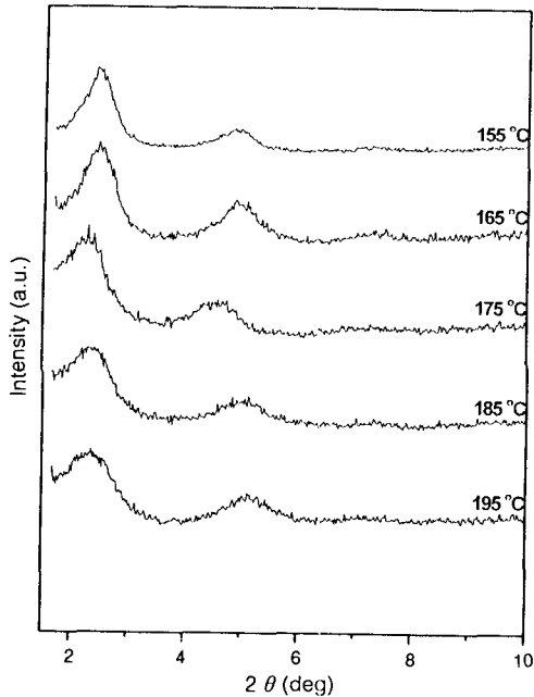
Figure 7. X-ray diffraction spectra of polystyrene/10A organosilicate hybrid at different annealing temperatures.
