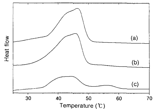
Figure 3. DSC thermograms of organosilicate MMT-2C 18 with different packing density : (a) 6A (CEC 140), (b) 15A (CEC 125), and (c) 20A (CEC 95).
