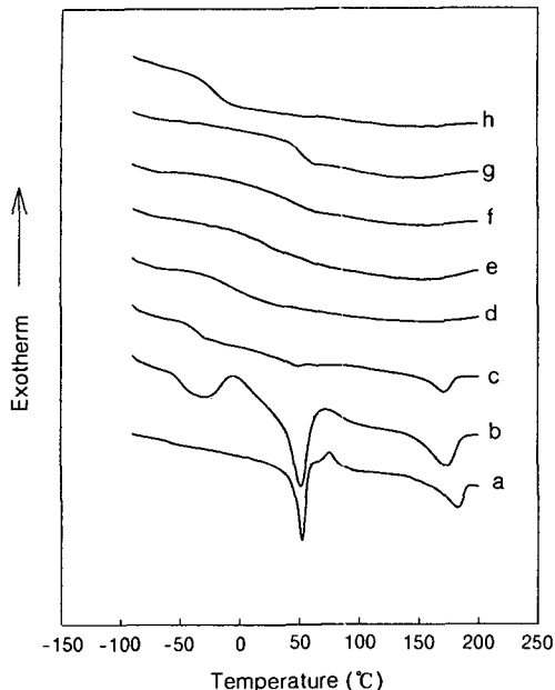
Figure 1. DSC thermograms obtained on heating of PCL-polyamide block copolymer/PVC blends ((a) 100/0, (b) 90/10, (c) 70/30, (d) 50/50, (e) 30/70, (f) 10/90, (g) 0/100 by weight) and (h) PCL homopolymer/PVC blends (50/50 by weight).
