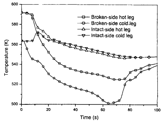
Fig. 8. Coolant Temperature Behaviors
