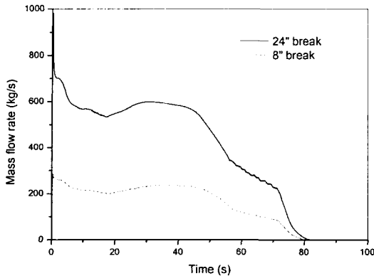
Fig. 5. Break Flow Behaviors
