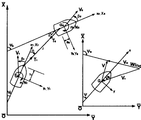
Fig. 1 Coordinate systems
