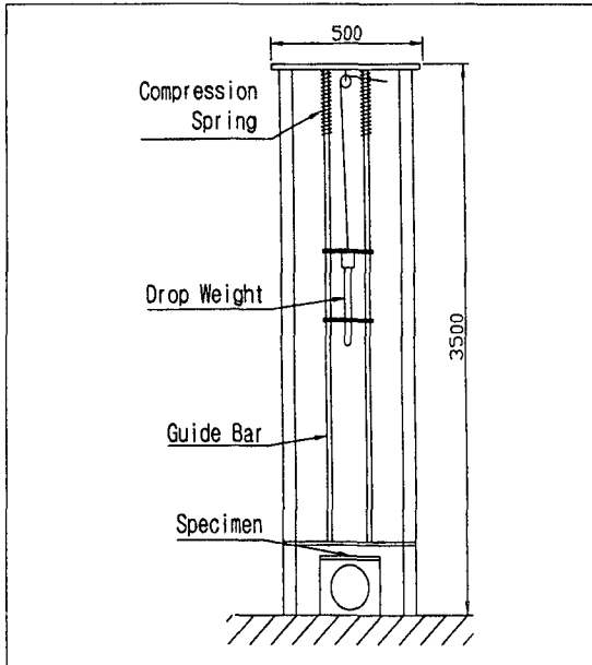
Fig. 1 Schematic diagram of falling weight tester
