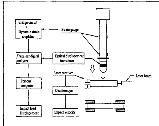
Fig. 2 Measurement system
