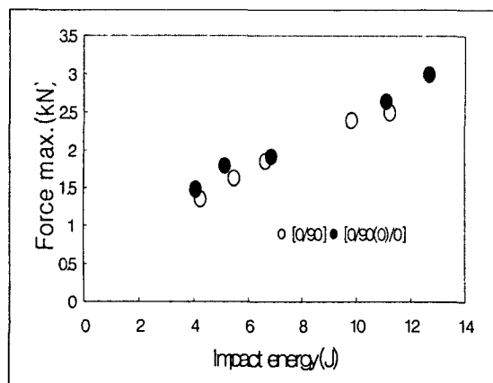
Fig. 12 Relation between maximum load and impact energy (specimen [0/90] A, specimen [0/90(0)/0] D)
