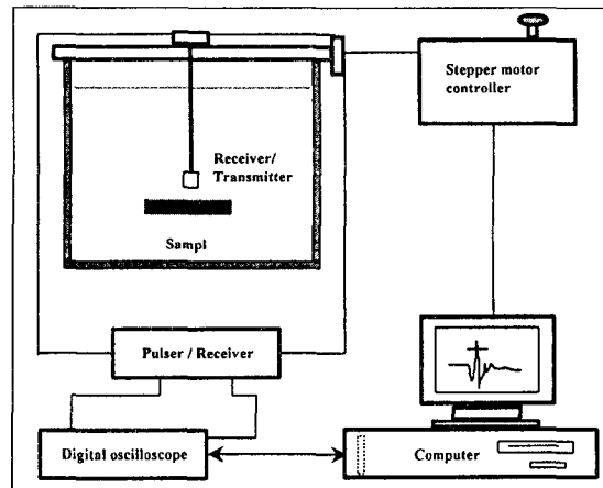
Fig. 3 Experimental setup for pulse-echo scan mode in immersion tank
