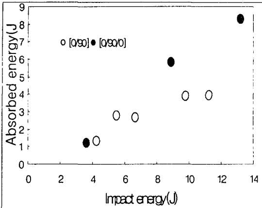
Fig. 9 Relation between absorbed energy and impact energy (specimen [0/90] A, specimen [0/90/0] C)
