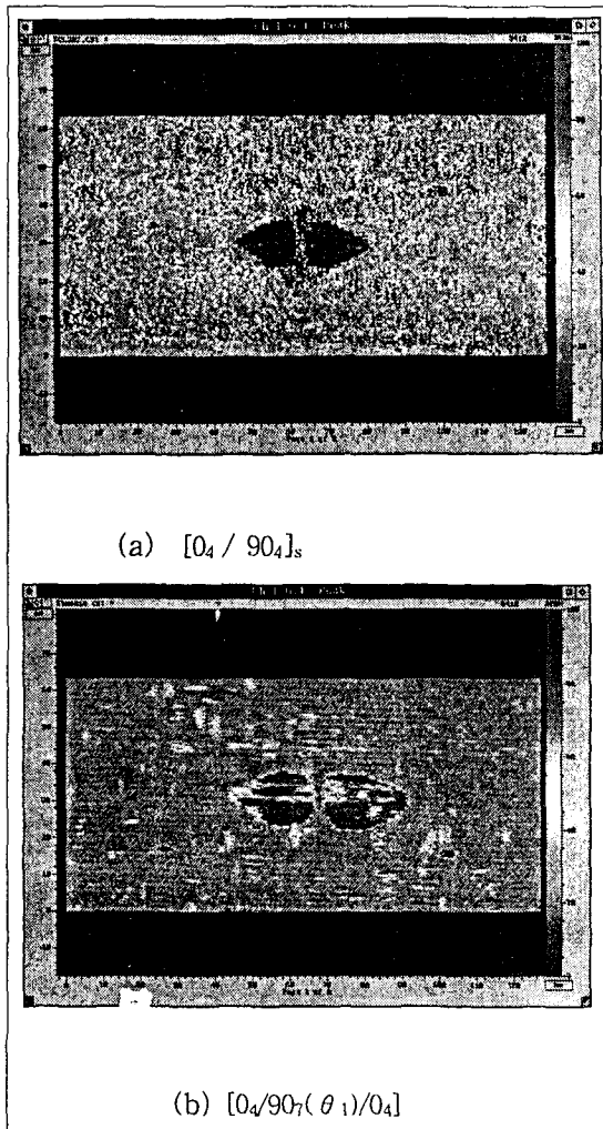
Fig. 6 Typical delamination shapes of specimens [0_4 / 90_4]_s and [0_4 / 90_7(\theta_1) / 0_4] on the rear side of impact point
