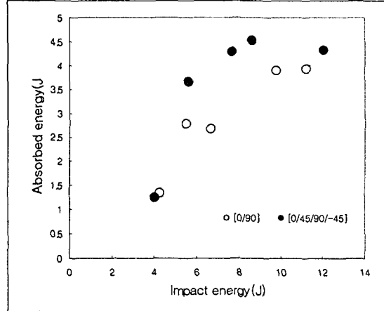
Fig. 7 Relation between absorbed energy and impact energy (specimen [0/90] A, specimen [0/45/90/-45] B)
