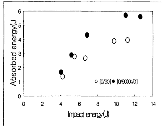
Fig. 11 Relation between absorbed energy and impact energy (specimen [0/90] A, specimen [0/90(0)/0] D)
