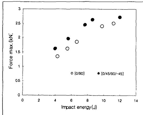
Fig. 8 Relation between maximum load and impact energy (specimen [0/90] A, specimen [0/45/90/-45] B)
