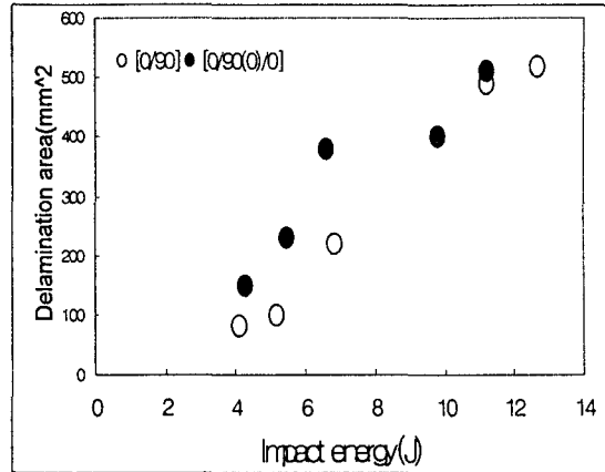
Fig. 14 Relation between impact energy and delamination area of specimens A and D
