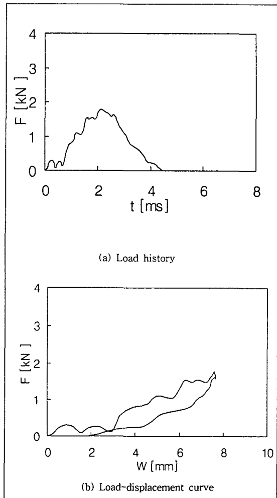
Fig. 5 Falling-weight test of CL2(Impact energy : 5.74J)
