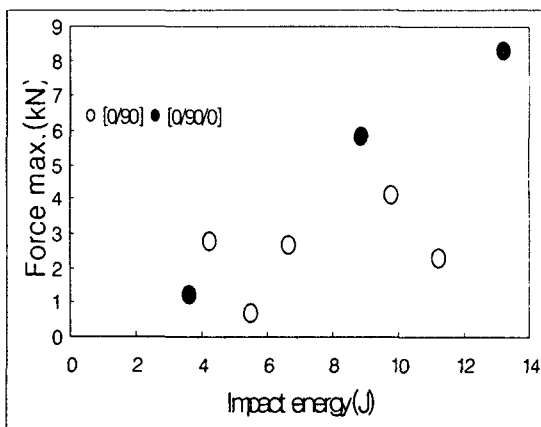
Fig. 10 Relation between maximum load and impact energy (specimen [0/90] A, specimen [0/90/0] C)
