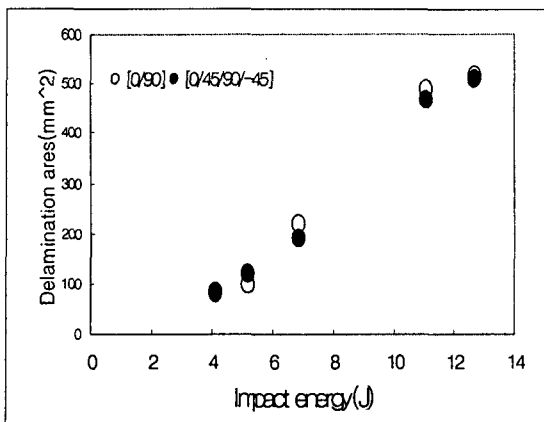
Fig. 13 Relation between impact energy and delamination area of specimens A and B
