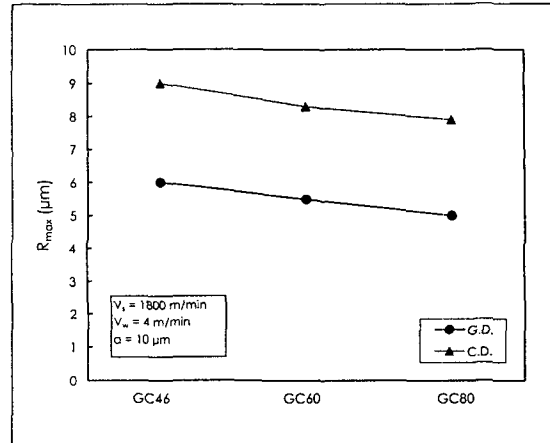
Fig. 6 Surface roughness versus grinding wheel grain in grinding direction (G.D.) and cross direction (C.D.) measured
