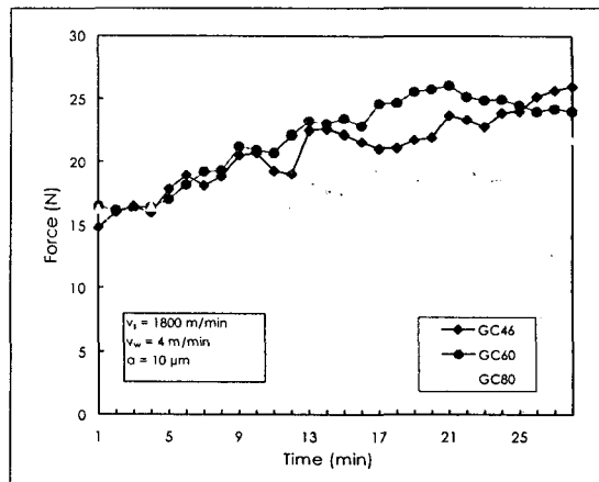
Fig. 5 Grinding force in surface grinding
