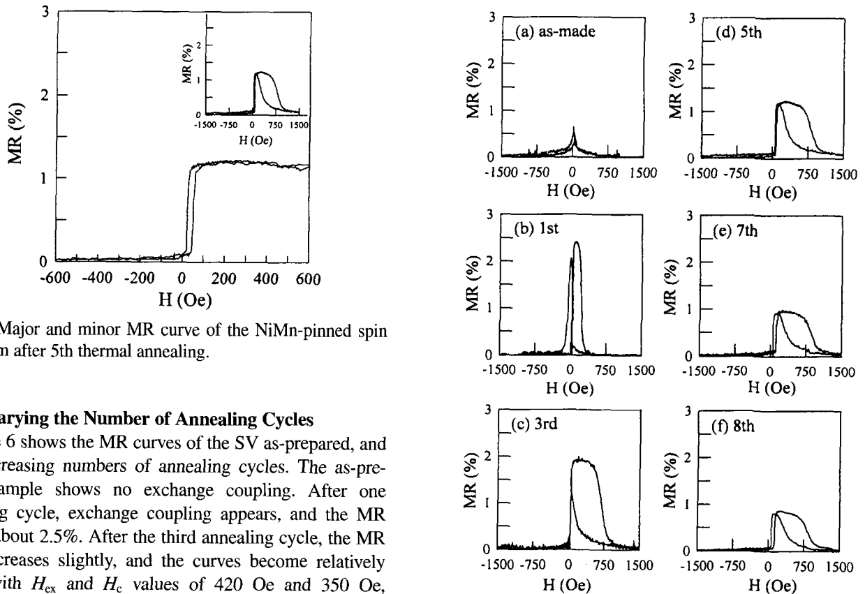
Fig. 6. MR curves of the spin valve film with annealing cycles.
