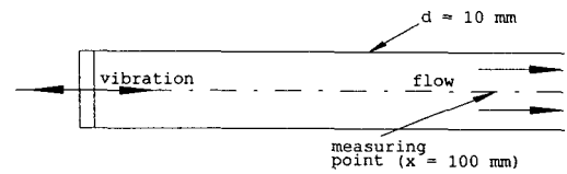
(a) Pipe flow with acoustic vibration
