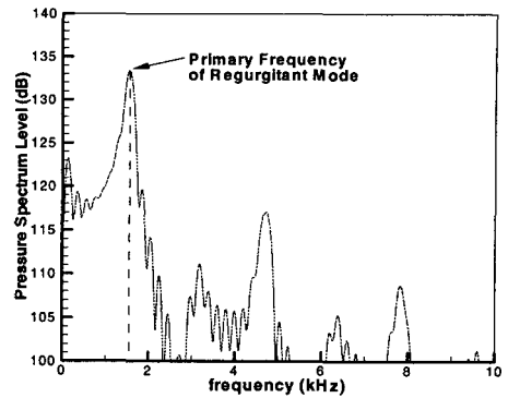
Figure 4a-f. Regurgitant mode of a tube in the subsonic flow, \bar{M} = 0.5 .
