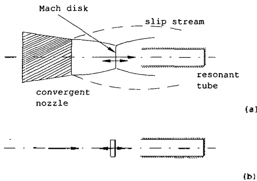
Figure 8a-b. Comparison of real physics and this model: (a) Hartmann-Sprenger tube, (b) the present problem.
