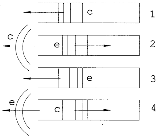
Figure 2. Schematic for resonating cycle of jet regurgitant mode where c is compressive wave and e is expansive wave.
