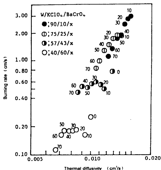
Fig. 8 Relationship between burning rate and thermal diffusivity of the W-KClO 4 -BaCrO 4 delay combustion
