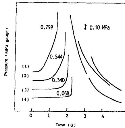
Fig. 4 Effect of loading on the pressure rise in the space before the combustion wave of the W-KClO_4-BaCrO_4 delay Composition ; W/KClO_4/BaCrO_4 = 30/25/45 (by weight), loading density ; (1) 50%, (2) 60%, (3) 70% and (4) 80% of theoretical maximum density
