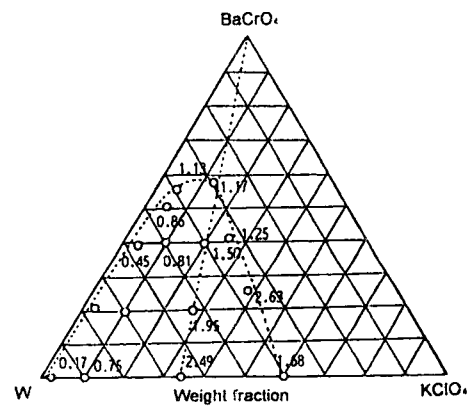
Fig. 7 Heat of combustion of the W-KClO 4 -BaCrO 4 delay composition (kJ/mol)
