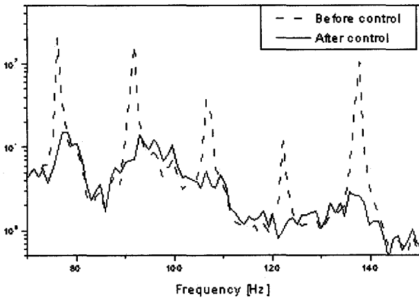
Fig. 8 Power spectra of the cabin noise of a passenger ship before and after control
