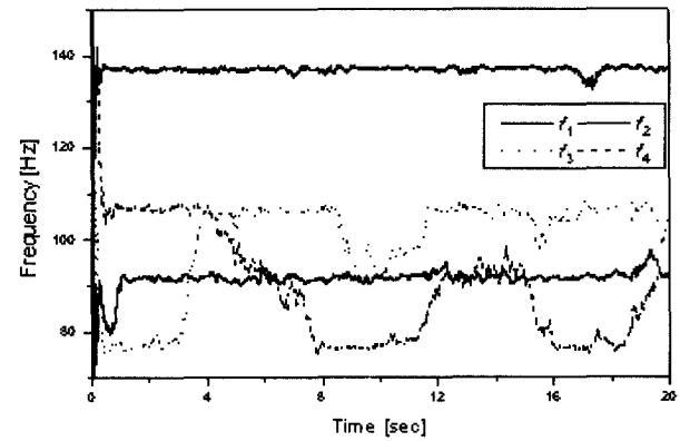
Fig. 4 Estimated frequencies drifted due to beating phenomena.
