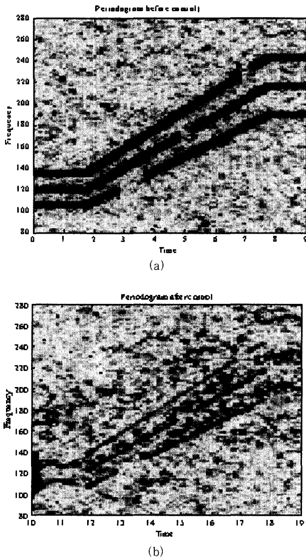
Fig. 12 Periodograms of time-varying signal with beating phenomena (a) before and (b) after control
