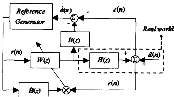
Fig. 7 Block diagram of ANC with reference generator
