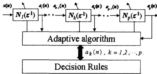
Fig. 5 The schematic diagram of the frequency estimation method with decision rules.
