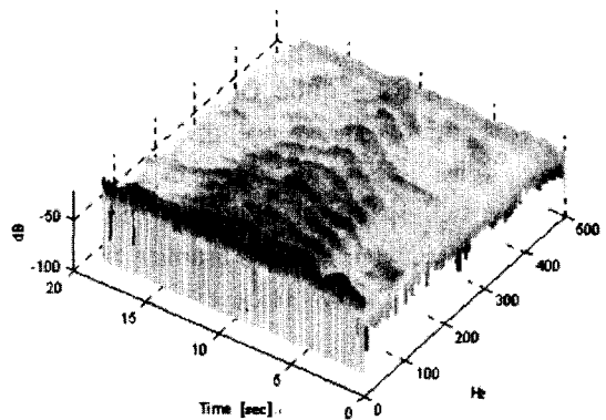
Fig. 10(b) Waterfall of the engine booming noise after control
