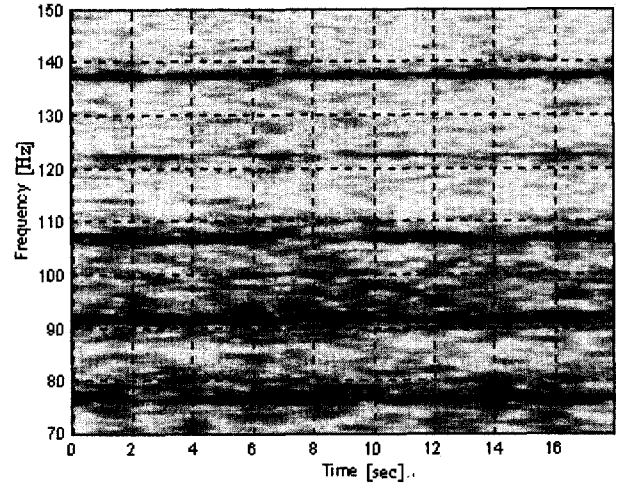
Fig. 3 Periodogram of cabin noise of a passenger ship.
