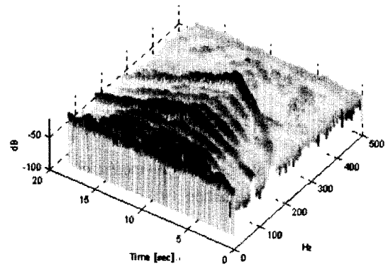
Fig. 10(a) Waterfall of the engine booming noise before control
