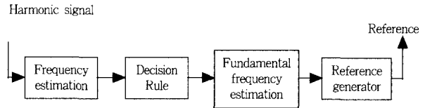
Fig. 6 The schematic diagram of the reference generation method.
