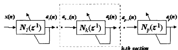
Fig. 1 Block diagram of the cascade ANF method.
