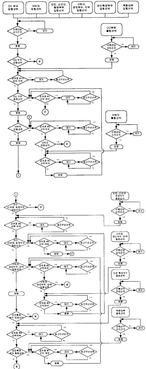
Fig. 3 Flow Chart to evaluate the Traffic Congestion in Channels
