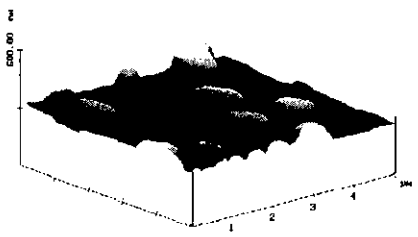
(b) Electrochemical etch-stopped Si surface.
