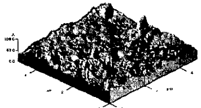
(b) TMAH 20 wt.%/IPA 17 vol.%.
