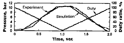
(b) Dynamic Characteristics of PCSV
