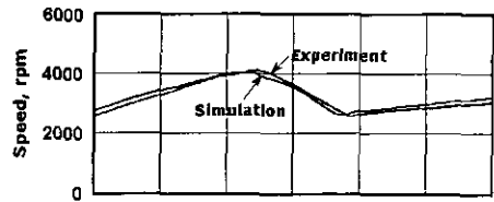
(c) Turbine speed
