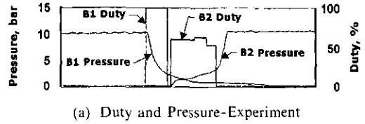
(a) Duty and Pressure-Experiment
