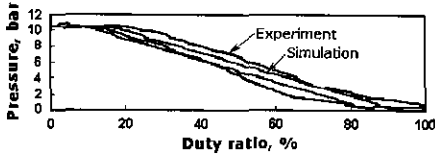
(c) Dynamic Characteristics of PCSV
