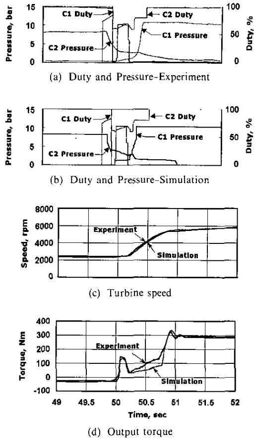
Fig. 11 Responses for 4-2 downshift
