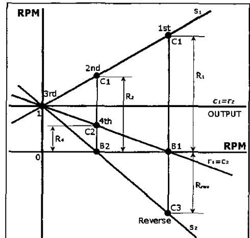
Fig. 7 R-R chart
