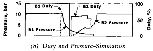
(b) Duty and Pressure-Simulation
