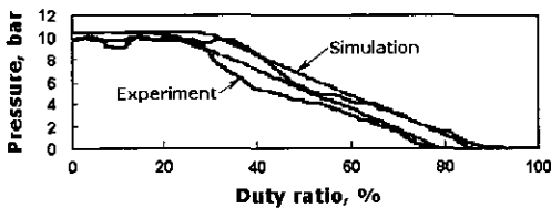
(c) Dynamic Characteristics of PCV for Sweep Frequency 0.5Hz
