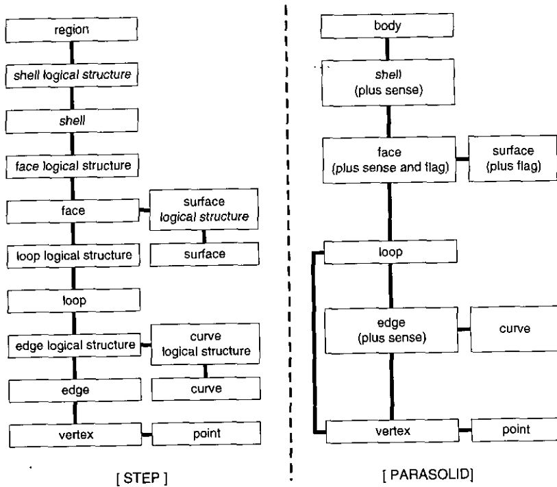
Fig. 2 Entity structures of STEP AP203 and Parasolid
