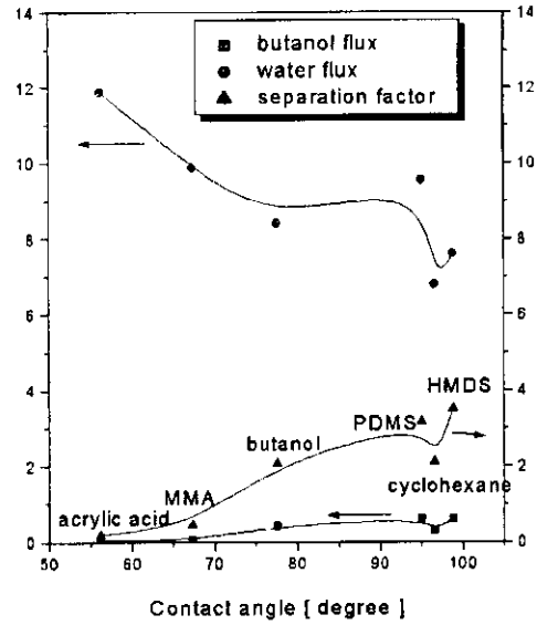
(feed : 3 wt.% butanol solution; feed flow rate : 36 liter/hr) Fig. 7. Effect of contact angle on flux and separation factor of butanol using plasma treated PP membrane.
