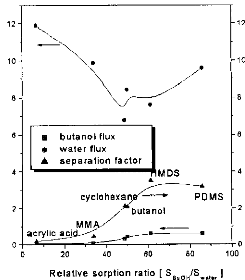
(feed : 3 wt.% butanol solution; feed flow rate : 36 liter/hr) Fig. 8. Effect of relative sorption ratio on flux and separation factor of butanol using plasma treated PP membrane.
