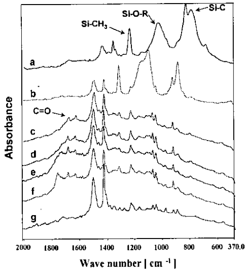
(A) hexamethyldisilane (B) poly(dimethyl siloxane) (C) cyclohexane (D) butanol (E) methylmethacrylate (F) acrylic acid (G) untreated PP Fig. 5. FT-IR(ATR) spectra of plasma treated PP surface.
