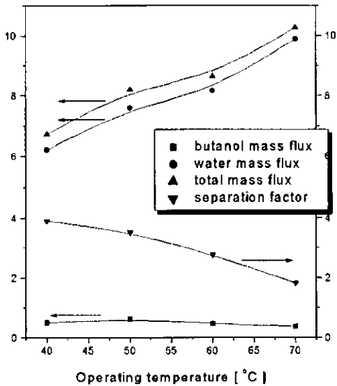
(feed : 3 wt.% butanol solution; feed flow rate : 36 liter/hr) Fig. 6. Effect of operation temperature on flux and separation factor of butanol using plasma treated PP membrane with hexamethyldisilane.
