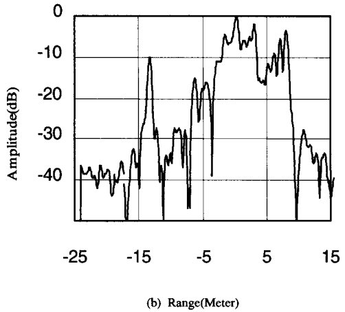
Fig. 4 Consecutive range profiles after accumulation.
