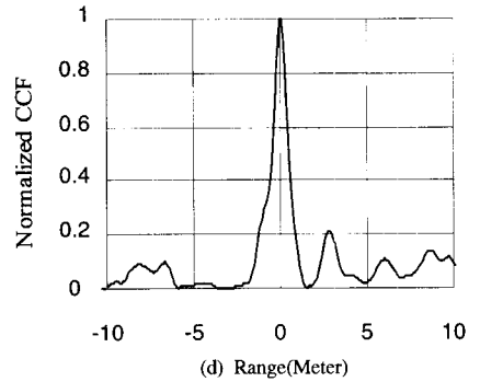
Fig. 2 CCF of range profiles. (a) CCF of two range profiles. (b) CCF with limitation. (c) CCF with accumulation. (d) CCF with limitation and accumulation.
