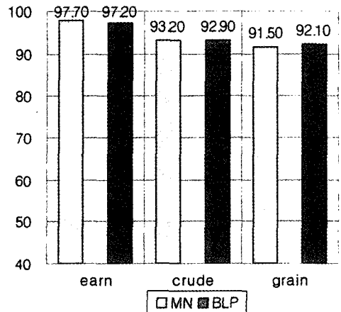
Fig. 3. Comparison of precision performances between multilayer perceptrons and BLP.
