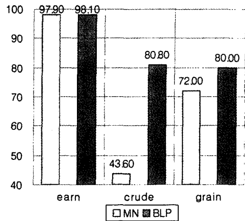
Fig. 2. Comparison of recall performances between multilayer perceptrons and BLP.
