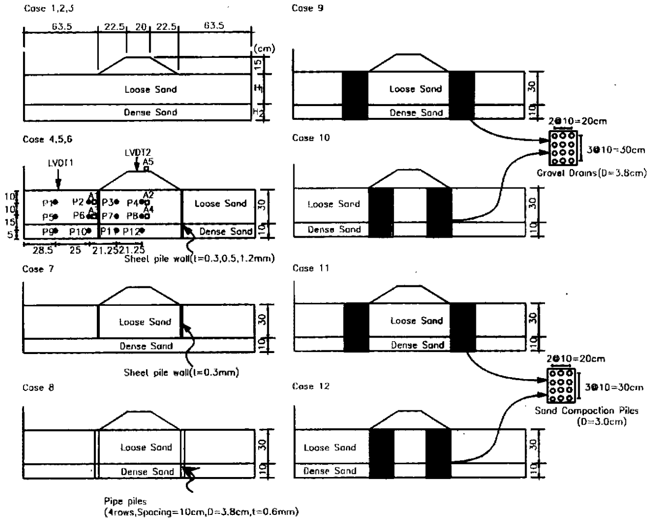
Fig. 1 Schematic drawings of each test set-up
