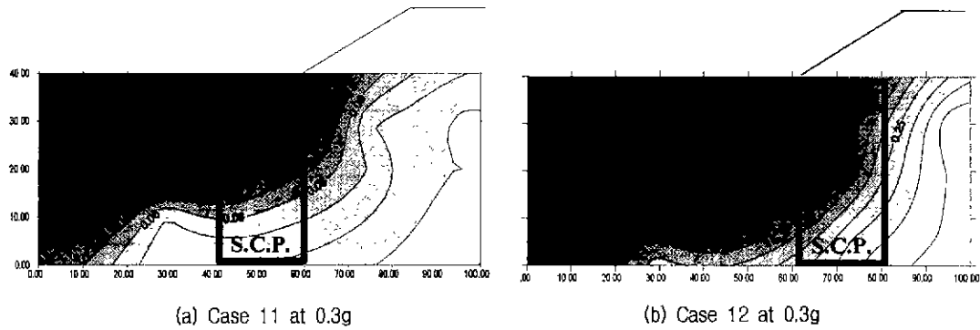
Fig. 5 Contours of excess pore water pressure ratios
