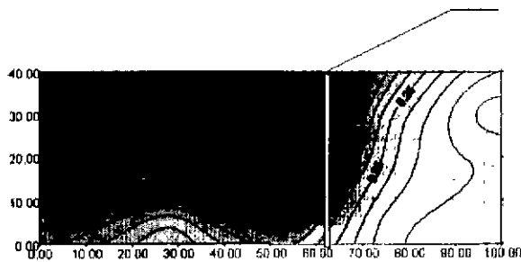
Fig. 3 Contours of excess pore water pressure ratios for case 6 at 0.15g
