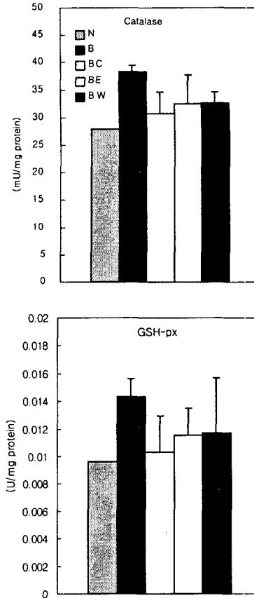
Fig. 3. Catalase and GSH-px activities of liver in rabbit fed atherogenic diet containing solvent fraction of kimchi for 16 weeks.
