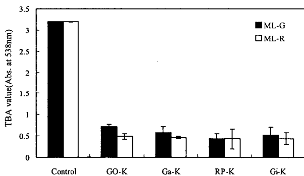
Fig. 1. Changes of TBA values of model systems of the different spices added mustard leaf during the reaction at 4°C for 4weeks.
