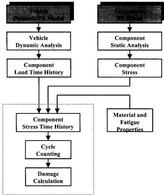
Fig. 1 Durability analysis procedure
