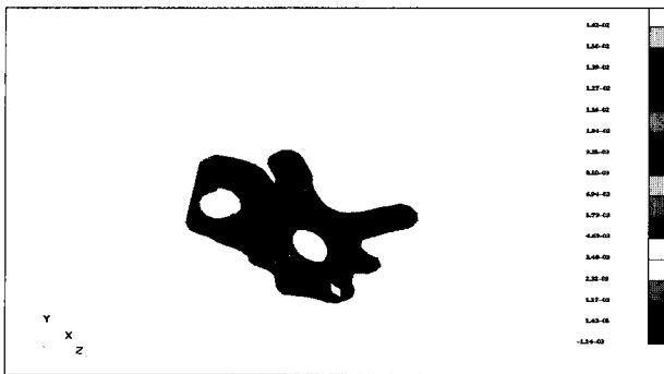
Fig. 7 Stress contour plot of the knuckle due to y-direction load
