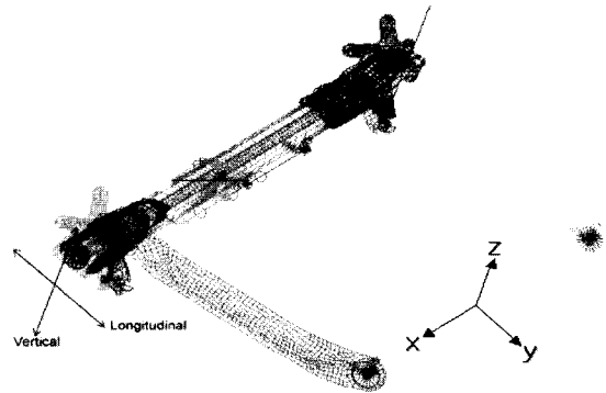
Fig. 3 Finite element model of the rear suspension
