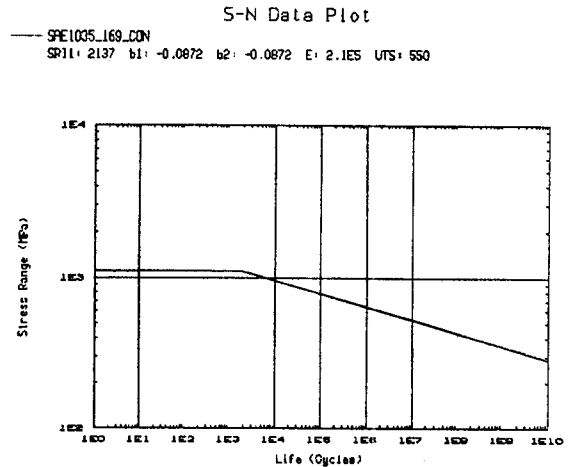
Fig. 8 S-N curve for SAE1035-169-CON
