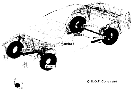
Fig. 2 Flexible vehicle dynamic model
