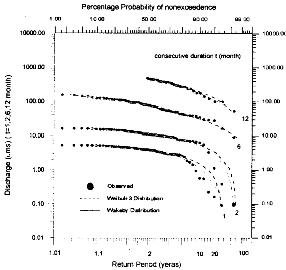
Fig. 1. Comparison of design low flow estimated using L-moments with Weibull plotting position for each consecutive duration at Jindong watershed of Nagdong river.
