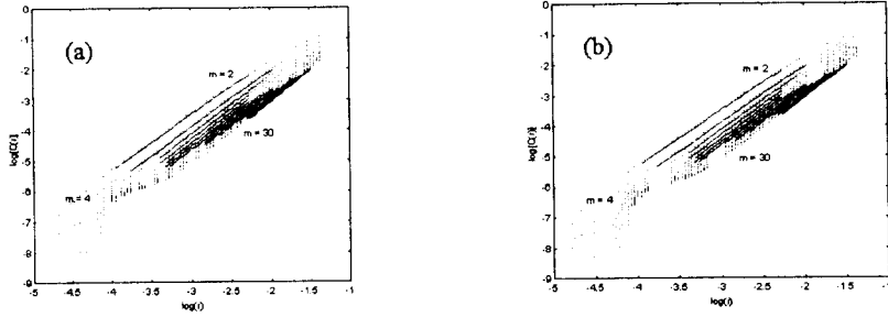
Fig. 3. Correlation integrals for 20000 data points generated from the Lorenz system of Eq. (15) using (a) \tau_d = 18 \tau_s and (b) \tau_w = 123 \tau_s .
