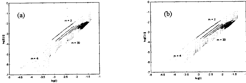
Fig. 5. Correlation integrals for 3000 data points generated from the Lorenz system using (a) \tau_d = 18 \tau_s and (b) \tau_w = 123 \tau_s .
