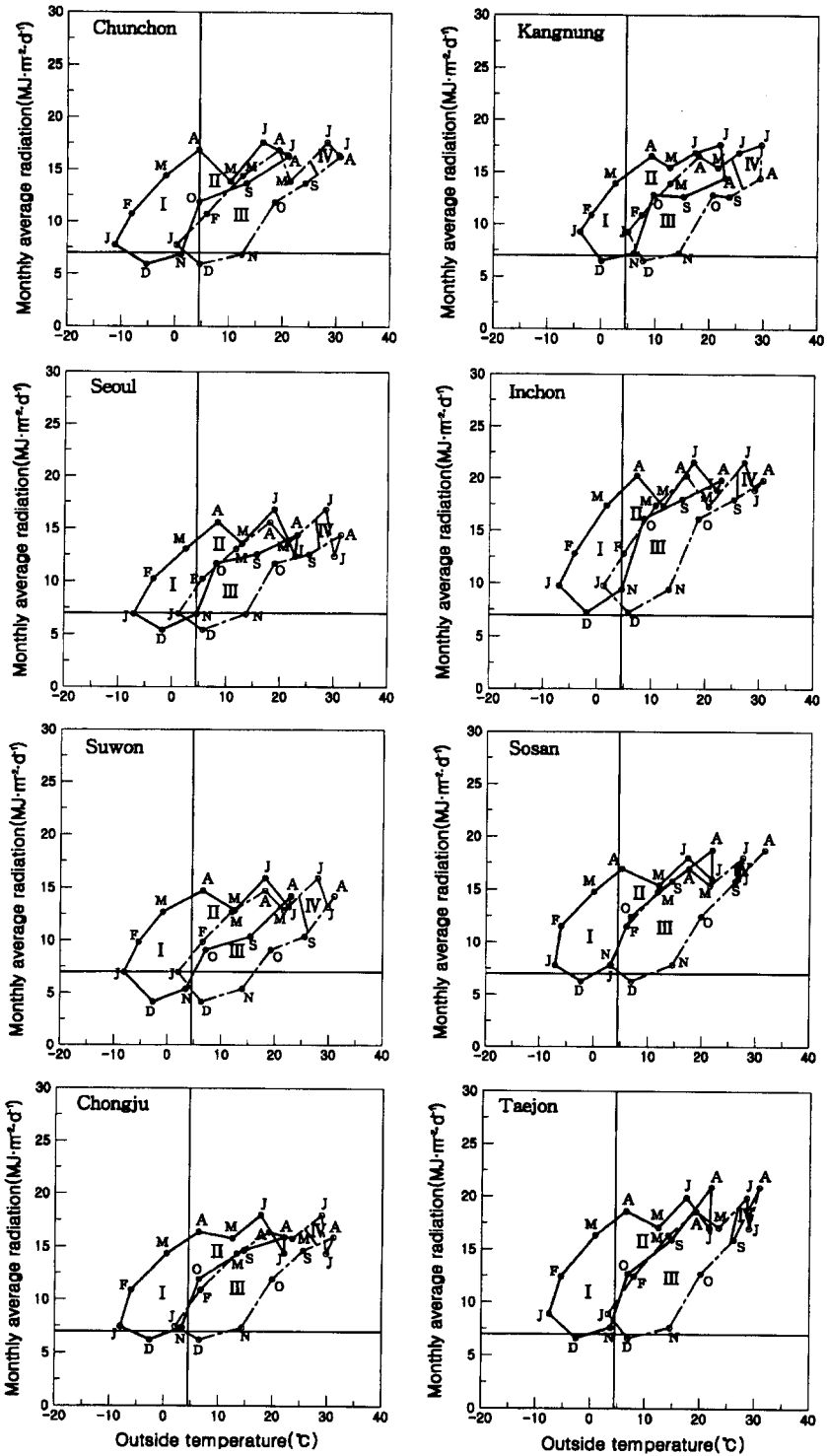
Fig. 1. Climographs for cucumber cultivation in plastic greenhouse.
