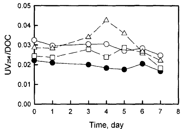
Fig. 5. Effect of biofiltration on UV 254 /DOC ratio with EBCT change in biofiltration experiment. (●: feed, ○: EBCT=10 min, □: EBCT=20 min, △: EBCT=40 min)
