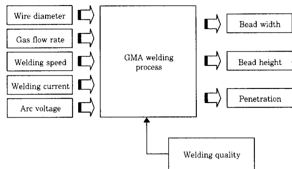
Fig. 1 Input and output parameters of the GMA welding process
