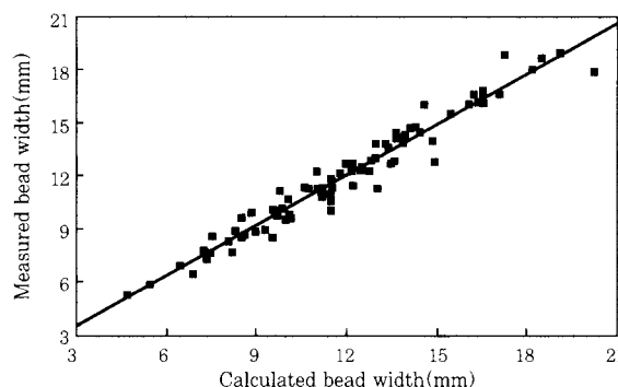
Fig. 4 Comparison of measured and calculated bead width using curvilinear equation
