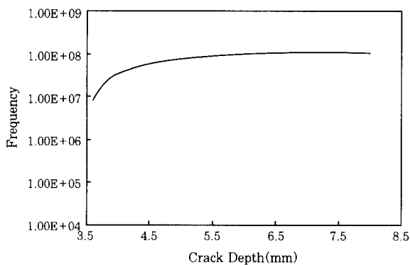
Fig. 7 Result of the crack propagation analysis of the butt joint welded lower flange
