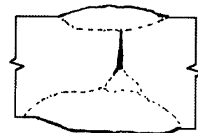
(a) Cross section of butt joint weld with IP
