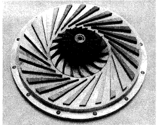
Fig. 1 Figure of test impeller and channel diffuser
