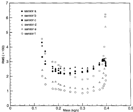
Fig. 8 Variations of RMS values of shaft unresolved component
