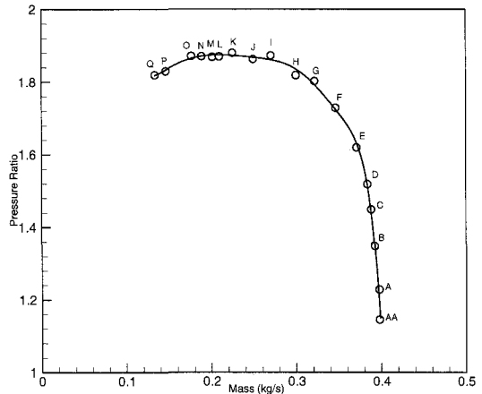
Fig. 4 Performance map at 60,000 rpm
