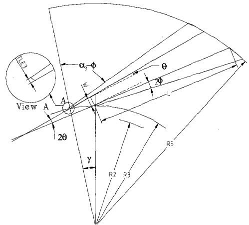
Fig. 2 Configurations and parameters of channel diffuser
