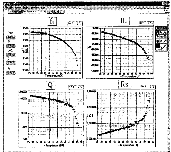
Fig. 3. A capture from the computer screen showing simultaneous display of temperature-dependent f_0 , IL , Q and R_S .
