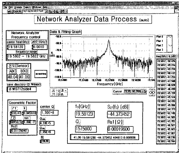
Fig. 2. A capture from the computer screen displaying the resonance peak, data for f_0 and IL , the fitted Q , and the calculated R_S .
