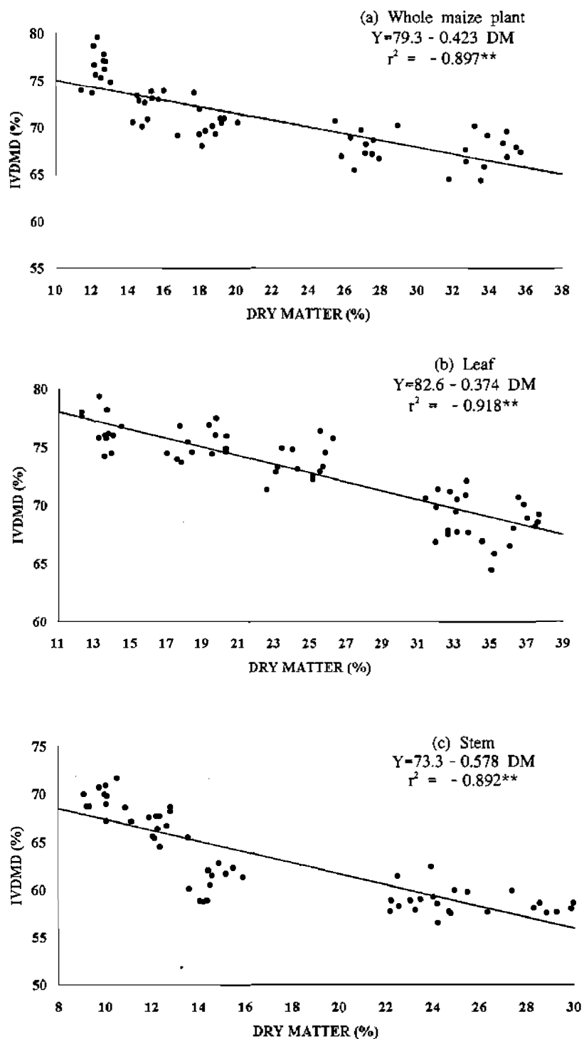
Figure 1. Relationship between in vitro IVDM and dry matter contents of whole maize plant (a), leaf (b) and stem (c)
