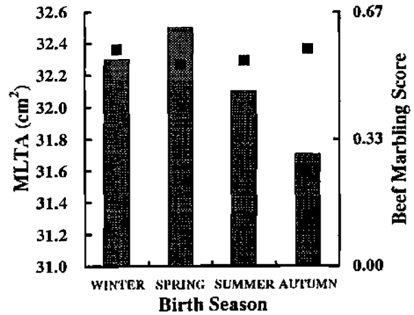
Figure 5. Ultrasonic estimates of MLTA and BMS of Japanese Brown Cows, by raising place
