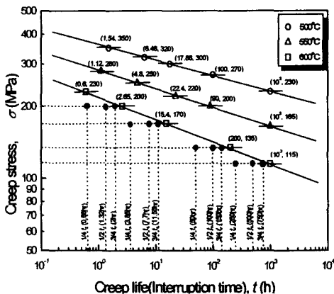
Fig. 8 Creep interruption curve(600°C)
