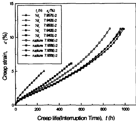
Fig. 7 Creep rupture curves (600°C, 105MPa)
