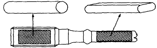
Fig. 2 Shape of ultrasonic test specimen
