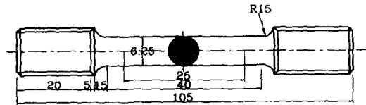
(c) High temperature tension test specimen (ASTM E21-79)
