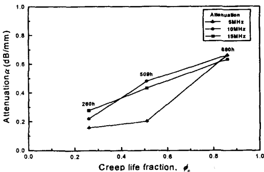
Fig. 12 Relationship of attenuation coefficient Vs. creep life fraction(creep test condition: 600°C, 105MPa, virgin material attenuation coefficient, a : 0.1015\text{dB/mm} )
