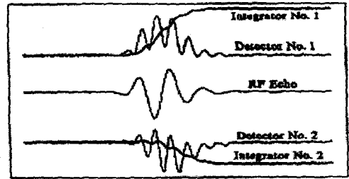
Fig. 4 Receiving and intergrating process versus phase angle of RF signal
