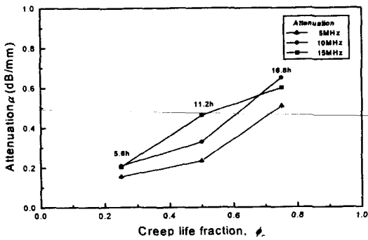
Fig. 11 Relationship of attenuation coefficient Vs. creep life fraction(creep test condition: 550°C, 220MPa, virgin material attenuation coefficient, a : 0.1015\text{dB/mm} )
