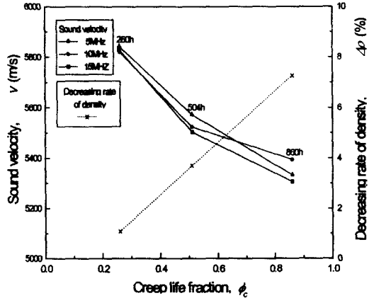
Fig. 10 Relationship of sound velocity and density Vs. creep life fraction(creep test condition: 600°C, 105MPa, virgin material sound velocity : 5,944m/s)
