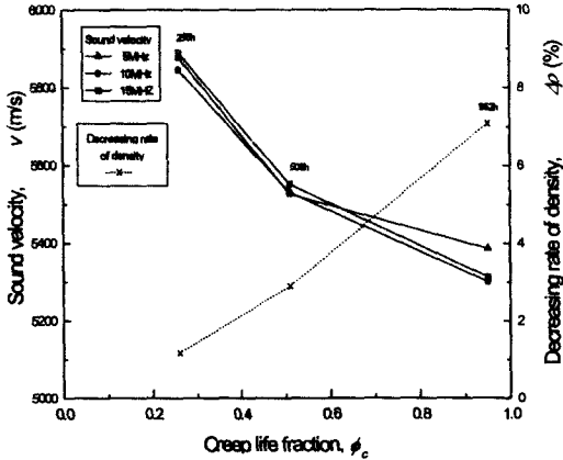
Fig. 9 Relationship of sound velocity and density Vs. creep life fraction(creep test condition: 550°C, 220MPa, virgin material sound velocity : 5,944m/s)
