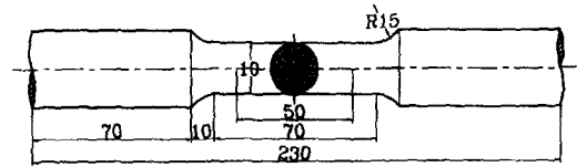
(b) Tension test specimen (KS B 0801 No.10 or ASTM 8-86)
