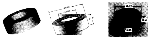
(a)3D Modeling (b)Dimensions (c)RP master
