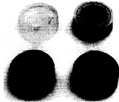
Fig. 4 Master model(upper,left), wax pattern(upper, right), casting part(lower,left: SUS304, lower, right : SNCM410)
