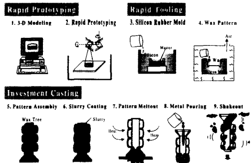
Fig. 1 Process of investment casting using rapid prototyping
