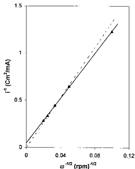
Figure 7. Koutecky-Levich plots for dioxygen reduction catalyzed by \text{Co}^{\text{II}}(\text{Br}_8\text{TTFP})(\text{Y})_2 in 0.05 M \text{H}_2\text{SO}_4 solution at 10 mV/s scan rate on a glassy carbon disk. The dashed line was calculated for the diffusion-convection limited reduction by two electrons.
