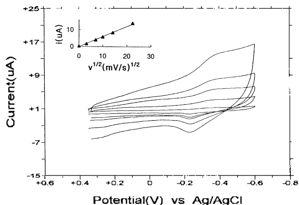
Figure 3. Cyclic voltammograms for the reduction of \text{Co}^{\text{II}}(\text{Br}_8\text{TTFP})(\text{Y})_2 in 0.05 M \text{H}_2\text{SO}_4 aqueous solution on the glassy carbon as a function of scan rate (10, 50, 100, 200, 500 mV/s). The inside plot represents the analysis of peak current vs (scan rate) ^{1/2} for the couple of \text{Co}^{\text{II}}/\text{Co}^{\text{I}} .
