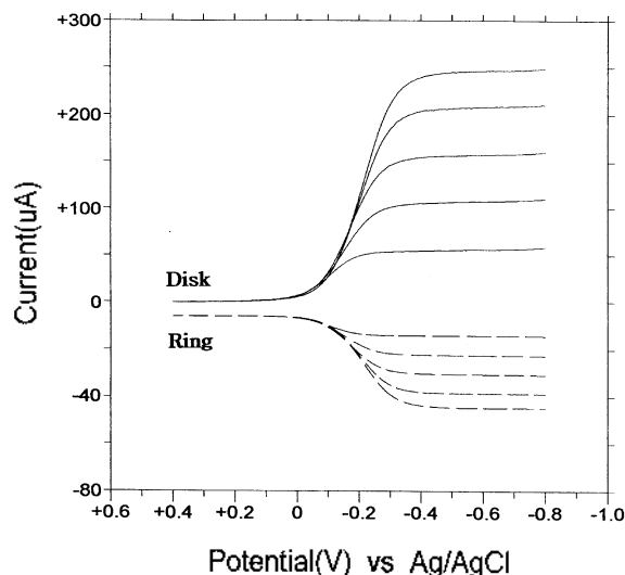
Figure 6. RRDE voltammograms ( E_r = +1.0 V) of dioxygen reduction for an dioxygen-saturated solution of \text{Co}^{\text{II}}(\text{Br}_8\text{TTFP})(\text{Y})_2 in 0.05 M \text{H}_2\text{SO}_4 solution at 10 mV/s scan rate. the rotation rates are 100, 400, 900, 1600, and 2500 rpm.
