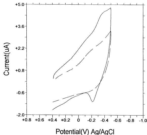
Figure 2. Cyclic voltammograms for the reduction of Co II (Br 8 TTFP)(Y) 2 in 0.05 M H 2 SO 4 aqueous solution on the glassy carbon (100 mV/s scan rate), for dissolved Co II (Br 8 TTFP)(Y) 2 (A); B: for dissolved 0.5 mM Co II (Br 8 TTFP)(Y) 2 (solid line) and for adsorbed Co II (Br 8 TTFP)(Y) 2 (dashed line).
