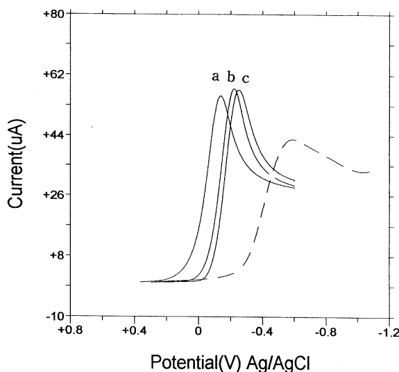
Figure 5. The effect of pH for the reduction potential of dioxygen in the presence of \text{Co}^{\text{II}}(\text{Br}_8\text{TTFP})(\text{Y})_2 : a: pH=1, b: pH=7, c: pH=10, dashed line: bare electrode at pH=1 in the absence of \text{Co}^{\text{II}}(\text{Br}_8\text{TTFP})(\text{Y})_2 .
