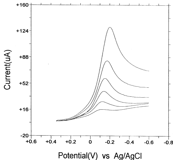
Figure 4. Cyclic voltammograms for the reduction of dioxygen in the presence of \text{Co}^{\text{II}}(\text{Br}_8\text{TTFP})(\text{Y})_2 in 0.05 M \text{H}_2\text{SO}_4 solution at different scan rates (10, 20, 50, 100, 200, 500 mV/s) on a glassy carbon electrode.
