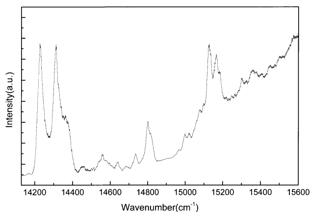
Figure 3. Excitation spectrum of \text{Cr}(\text{biuret})_3\text{Cl}_3 at 13K.
