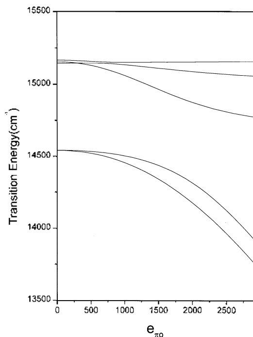
Figure 5. Calculated variation of the transition energies to the {}^2E_g and {}^2T_{1g} state for \text{Cr}(\text{biuret})_3^{31} as a function of e_{\pi o} .
