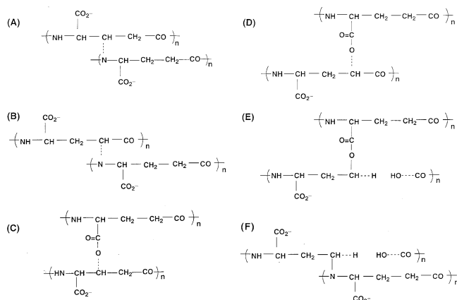
Figure 4. Some possible chemical bonds created due to cross-linking and hydrolysis created by radical reactions in PGA; only bonds between methylene or methine carbons and oxygen or nitrogen are shown. The chemical bonds are represented as dotted line.
