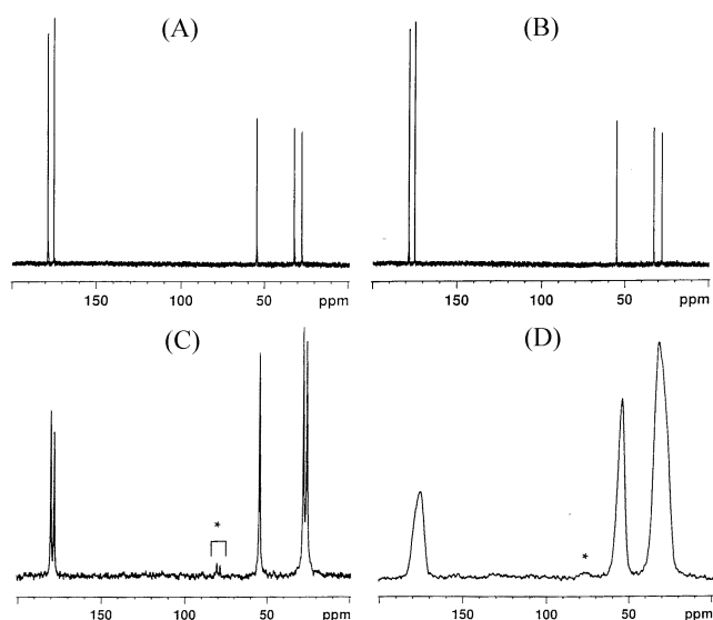
Figure 1. Liquid state 13 C NMR spectra of (A) GA and (B) PGA. Solid state 13 C CP-MAS spectra of (C) GA at 10 kHz and (D) PGA at 10 kHz. Spinning side bands are marked by *.
