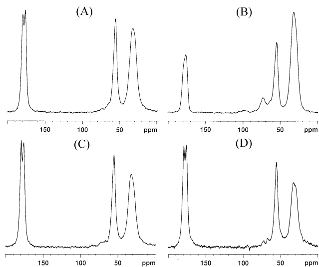
Figure 3. Solid state ^{13}\text{C} CP-MAS NMR spectra of (A) hydrolyzed PGA-90 kGy, (B) hydrolyzed PGA-170 kGy, (C) PGA-90 kGy, and (D) PGA-170 kGy. All spectra were obtained at the spinning rate of 12.5 kHz.
