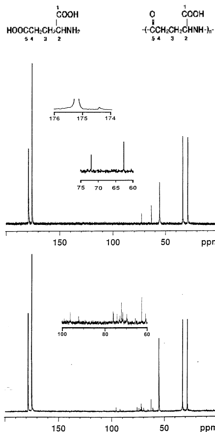
Figure 2. Liquid state 13 C NMR spectra of (A) hydrolyzed PGA-90 kGy and (B) hydrolyzed PGA-170 kGy. Regions with small peaks are expanded as in insets.
