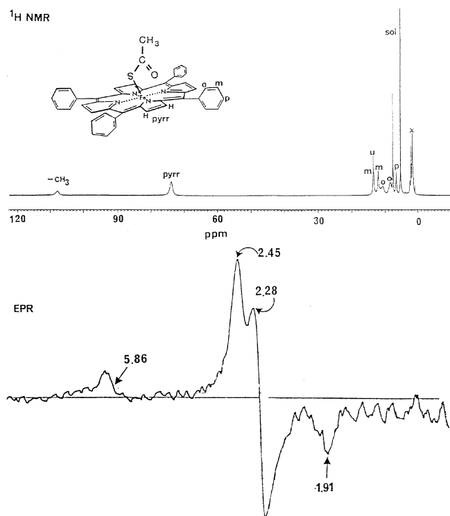
Figure 2. 1 H NMR (360 MHz) and EPR spectra for the reaction of ( d_5 -TPP)Fe(III)O 3 SCF 3 with 1.0 equiv. [CH 3 C(=O)S] - K + /methanol in dichloromethane solution. EPR spectrum was recorded at 77 K with 6000 G sweep, 9.19 GHz, 100 KHz modulation at 5 mwatt.
