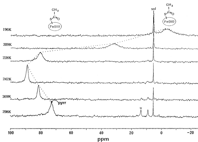
Figure 1. Deuterium NMR spectra for the reaction of 4.0 mM ( d_5 -TPP)Fe(III)O 3 SCF 3 with 1.0 equiv. [CH 3 C(=O)S] - K + /methanol in dichloromethane solution. A) 298 K, B) 269 K, C) 242 K, D) 228 K, E) 209 K, and F) 196 K. Denoted "u" indicate u-oxo dimeric species due to the contamination from the trace amount of oxygen present in solution.
