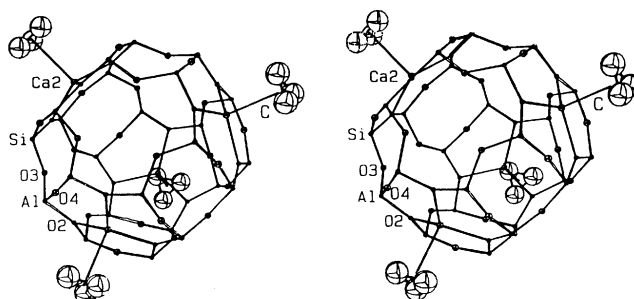
Figure 3. A stereoview of a sodalite cavity. Four \text{Ca}^{2+} ions, Ca(2), are shown at site II. Each \text{Ca}^{2+} ion at Ca(2) coordinates to one cyclopropane molecule. The hydrogen atoms, whose positions were not determined, are not shown. All D6Rs have this arrangement. At least 75% of sodalite cavities have this arrangement. The remaining 25% have only three \text{Ca}^{2+} ions at Ca(2), each of which coordinates to one cyclopropane molecule. Ellipsoids of 20% probability are shown.
