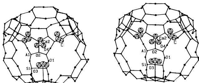
Figure 5. Stereoview of the supercage of the \text{C}_3\text{H}_6 complex of \text{Ca}_{46}\text{-X} . Four \text{Ca}^{2+} ions at ions at Ca(2) (site) are shown. Each coordinates to one cyclopropane molecule. Ellipsoids of 20% probability are used.
