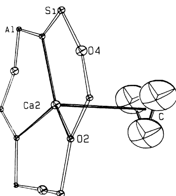
Figure 4. \text{Ca}(\text{C}_3\text{H}_6)_2^{2+} complex on the inner surface of a supercage is shown in stereoview. The positions of the hydrogen atoms were not determined. Ellipsoids of 20% Probability are shown.
