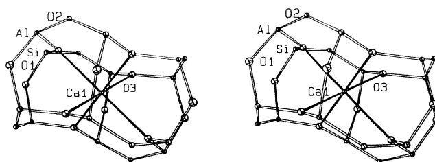
Figure 2. Stereoview of double six-ring of \text{Ca}_{10}\text{-X } 30\text{C}_3\text{H}_6 . The \text{Ca}^{2+} ion at Ca(1) is shown at site I. Ellipsoids of 20% probability are used.
