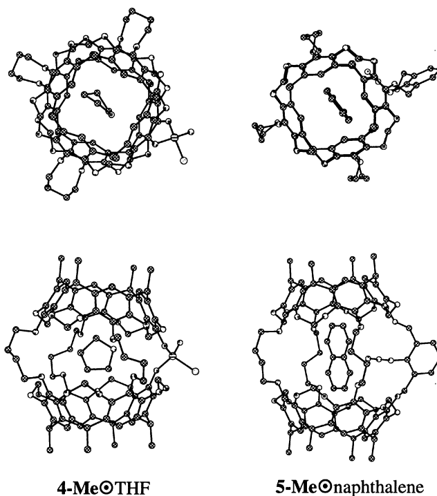
Figure 2. Optimized lowest energy structures of 4-Me@THF and 5-Me@naphthalene.
