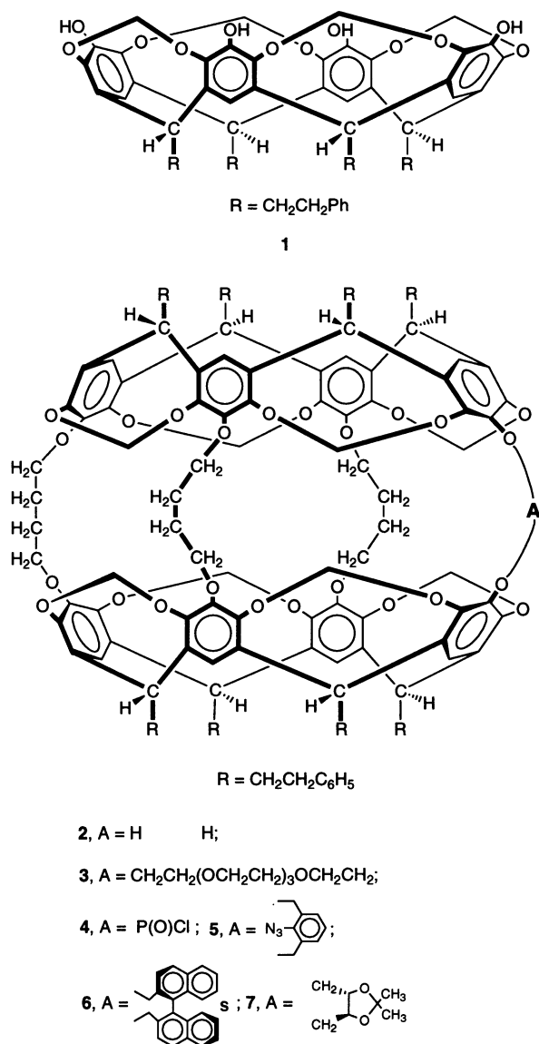
Figure 1. Structures of compounds 1-7.
