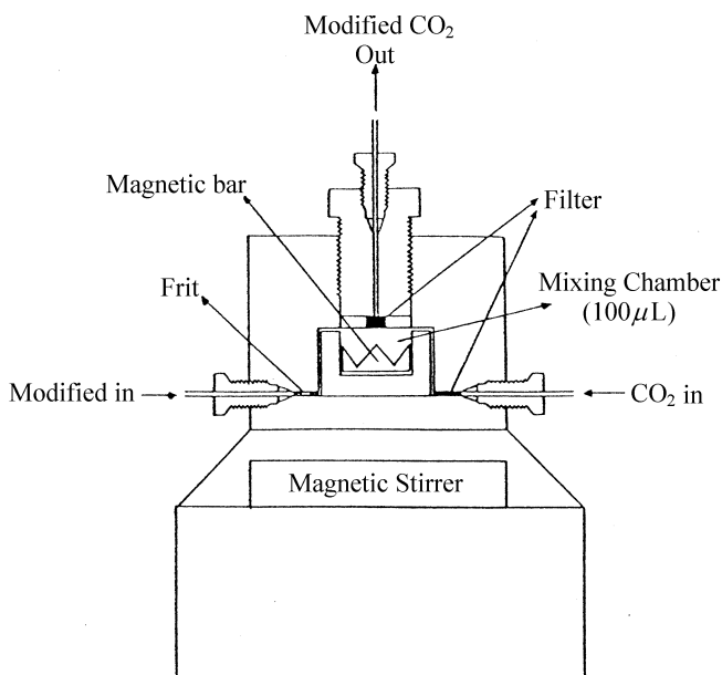
Figure 1. Mixing Device.
