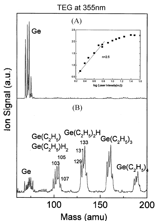
Figure 1. The MPI (355 nm)/TOF mass spectrum of TEG at (A) 2.1 kJ/cm 2 and (B) 2.3 J/cm 2 per pulse (see the text). The inset of (A) shows the log-log plot of the Ge ion signal vs. the laser intensity (mJ/pulse), whose slope is 2.5±0.1.
