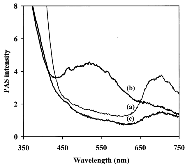
Figure 6. Photoacoustic spectra of (a) calcined MCM-41, (b) APTMS/MCM-41, and (c) AAPTMS/MCM-41 treated at room temperature for 1 h with Reichardt's dye solution ( 10 \text{ mL}, 10^{-3} \text{ M} ), respectively.
