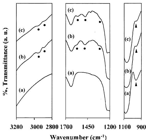
Figure 3. IR spectra of (a) calcined MCM-41, (b) APTMS/MCM-41, and (c) AAPTMS/MCM-41.
