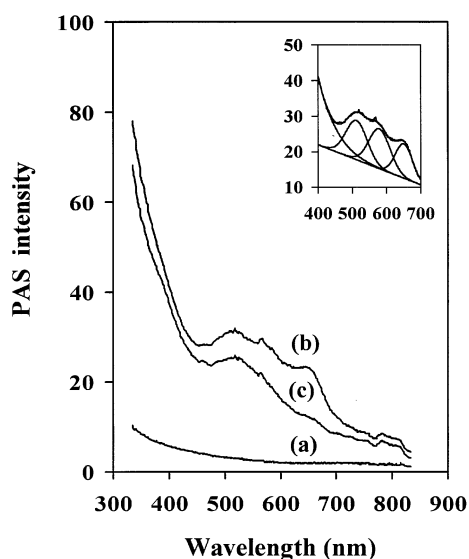
Figure 7. Photoacoustic spectra of (a) APTMS/MCM-41, (b) Co/APTMS/MCM-41, and (c) Co/AAPTMS/MCM-41. Inset shows the deconvoluted curves of PAS for Co/APTMS/MCM-41 by curve-fitting calculation.
