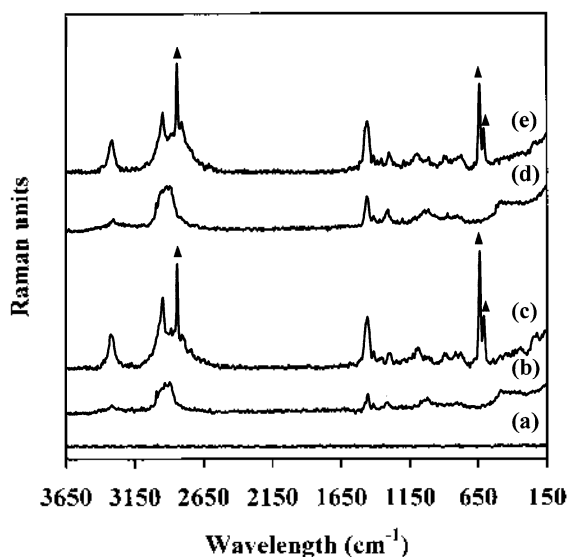
Figure 4. Raman spectra of (a) calcined MCM-41, (b) APTMS/MCM-41, (c) APTMS, (d) AAPTMS/MCM-41, and (e) AAPTMS.
