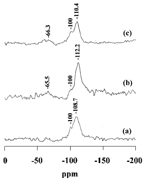
Figure 5. ^{29}\text{Si} MAS NMR spectra of (a) MCM-41, (b) APTMS/MCM-41, and (c) AAPTMS/MCM-41.
