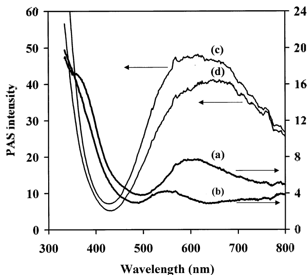
Figure 9. Photoacoustic spectra of (a) Ni/APTMS/MCM-41, (b) Ni/AAPTMS/MCM-41, (c) Cu/APTMS/MCM-41, and (d) Cu/AAPTMS/MCM-41.
