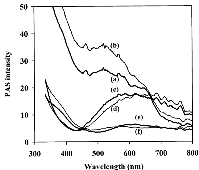
Figure 10. Photoacoustic spectra of (a) Co/APTMS/MCM-48, (b) Co/AAPTMS/MCM-48, (c) Cu/APTMS/MCM-48, (d) Cu/AAPTMS/MCM-48, (e) Ni/APTMS/MCM-48, and (f) Ni/AAPTMS/MCM-48.
