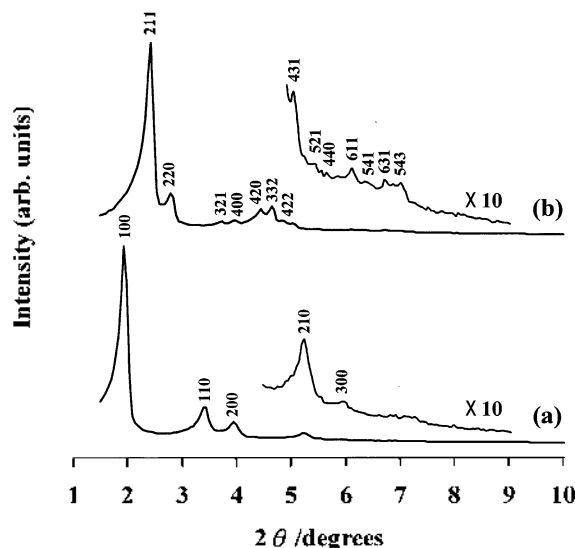
Figure 1. XRD patterns of (a) calcined MCM-41 and (b) calcined MCM-48.
