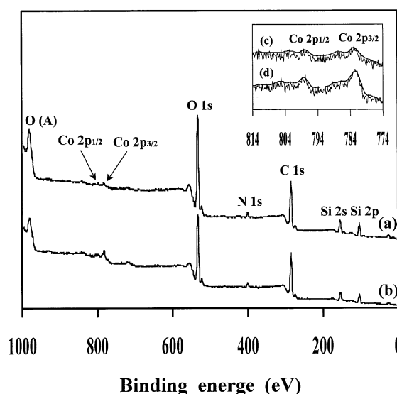
Figure 8. X-ray photoelectron spectra of (a) Co/APTMS/MCM-41 and (b) Co/AAPTMS/MCM-41. Inset shows the smoothed and enlarged XP spectra of the cobalt 2p photoelectron region of (c) spectrum (a) and (d) spectrum (b).
