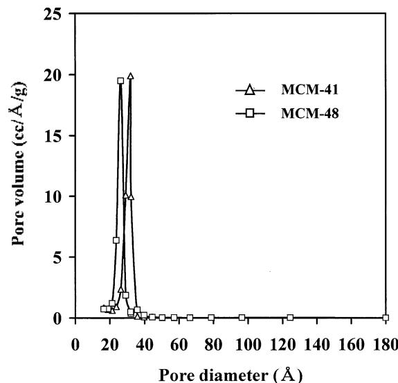
Figure 2. Pore size distribution curves of calcined MCM-41 and calcined MCM-48 calculated from the desorption branch of the nitrogen adsorption isotherm using the BJH formula.
