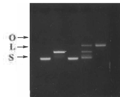
Figure 2. Cleavage of pAT by wild type EcoRV and Asp90Cys+Ile91Leu mutant on pAT153 in the presence of Mg^{2+} and Cu^{2+} . Reactions in buffer contained 10 nM DNA with either Mg^{2+} or Cu^{2+} . Lane 1 is supercoiled DNA without enzyme. The DNA was digested by wild type EcoRV (lane 2) and Asp90Cys+Ile91Leu mutant (lane 4) in the presence of Mg^{2+} and by wild type EcoRV (lane 3) and Asp90Cys+Ile91Leu mutant (lane 5) in the presence of Cu^{2+} , respectively. The mobilities of the supercoiled, open-circle, and linear forms of the plasmids are marked on the left of the gel as S, O, L, respectively.
