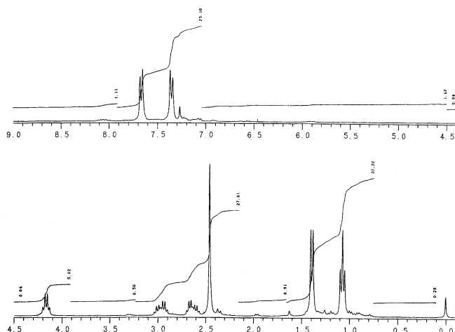
Figure 1. ^1\text{H} NMR spectrum of 3-toluenesulfonyl-2-pentene ( 9 ) (solv. \text{CDCl}_3 )
