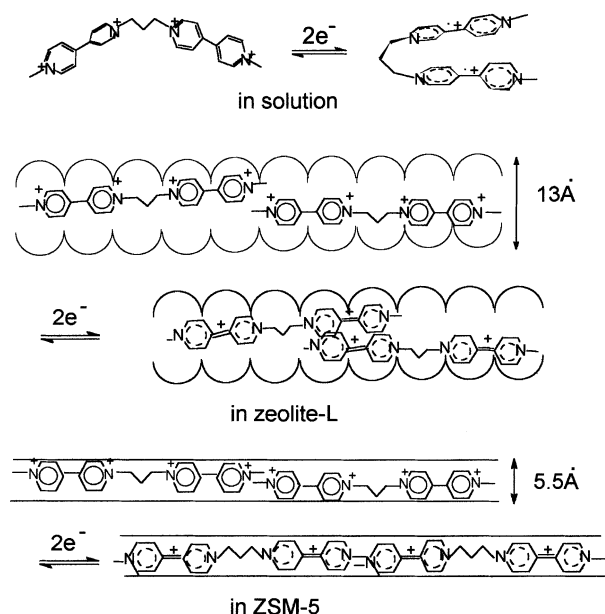
Figure 3. Schematic diagram for intramolecular dimerization of C_1V^+-C_3-VC_1^+ in solution (top), intermolecular dimerization in zeolite-L (middle), and suppression of dimerization of C_1V^+C_3-VC_1^+ in ZSM-5 (bottom).
