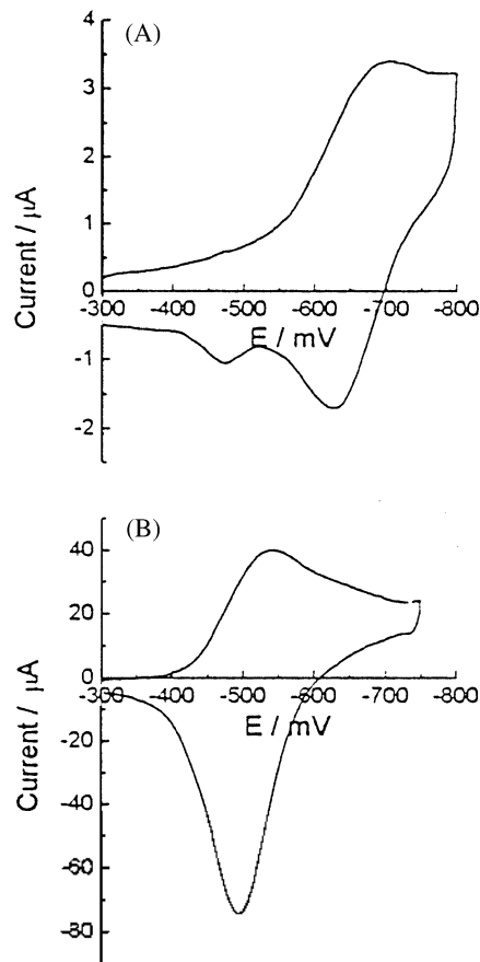
Figure 2. Cyclic voltammetric waves of C_1V^{2+}-C_3-VC_1^{2+} /zeolite-L modified electrode in 0.1 M KCl solution with scan rate of 0.1 V/s. Loading: 7.1 \times 10^{-6} mol/g (A); 1.7 \times 10^{-4} mol/g (B).
