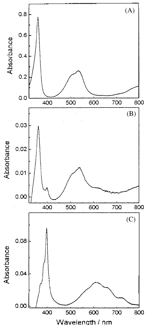
Figure 1. Absorption spectra of C_1V^{2+}-C_3-VC_1^{2+} in an aqueous solution (A, 1 mM), C_1V^{2+}-C_3-VC_1^{2+} incorporated into zeolite L (B, Loading: 1.4 \times 10^{-4} mol/g) and C_1V^{2+}-C_3-VC_1^{2+} incorporated into ZSM-5 in 0.1 M KCl solution (C, Loading: 1.7 \times 10^{-4} mol/g).
