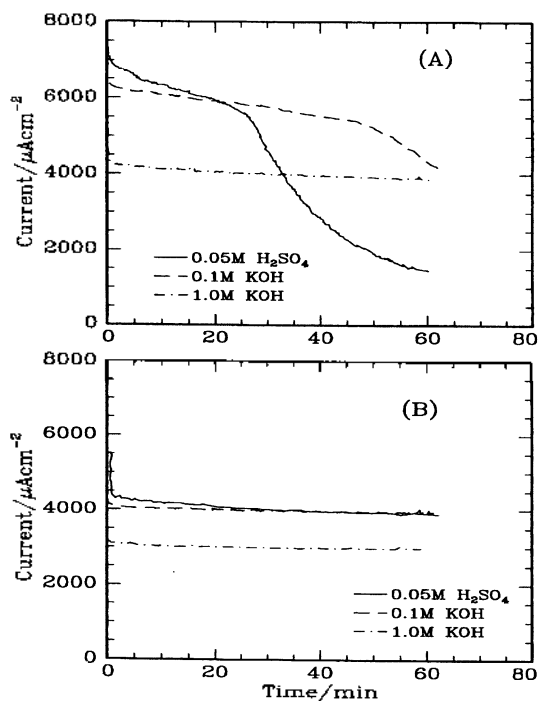
Figure 6. Changes in the limiting currents of oxygen reduction with time at PEDT-MTSP electrodes in O_2 -saturated solutions. (A) PEDT-FeTSP. (B) PEDT-CoTSP. The potential was fixed for diffusion-limited current in each case
