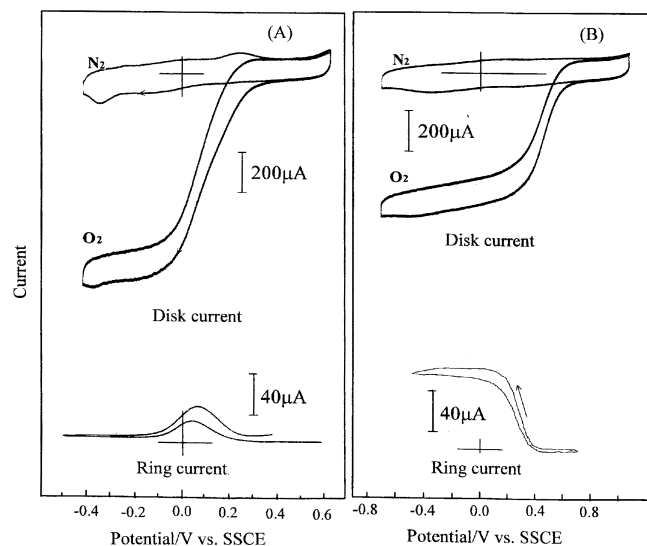
Figure 4. RRDE currents with oxygen reduction at PEDT-MTSP disk electrodes in O 2 -saturated 0.05 M H 2 SO 4 . (A) PEDT-FeTSP. (B) PEDT-CoTSP. Scan rate: 50 mV s -1 ; Rotation rate: 2000 rpm.
