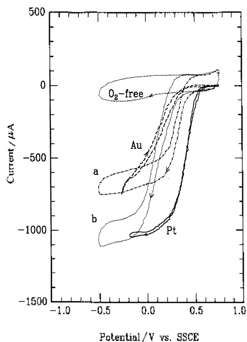
Figure 2. O 2 reduction currents at rotating PEDT-CoTSP (a), PEDT-FeTSP (b), Pt, and Au electrodes in O 2 -saturated 0.05 M H 2 SO 4 . Scan rate: 50 mV s -1 ; Rotation rate: 2000 rpm; Electrode area: 0.164 cm 2 .
