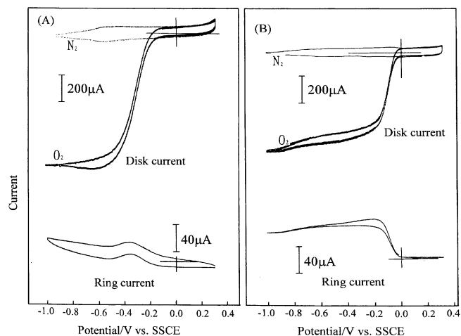
Figure 5. RRDE currents with oxygen reduction at PEDT-MTSP disk electrodes in O 2 -satd. 0.1 M KOH. (A) PEDT-FeTSP. (B) PEDT-CoTSP. Scan rate: 50 mV s -1 ; Rotation rate: 2000 rpm.
