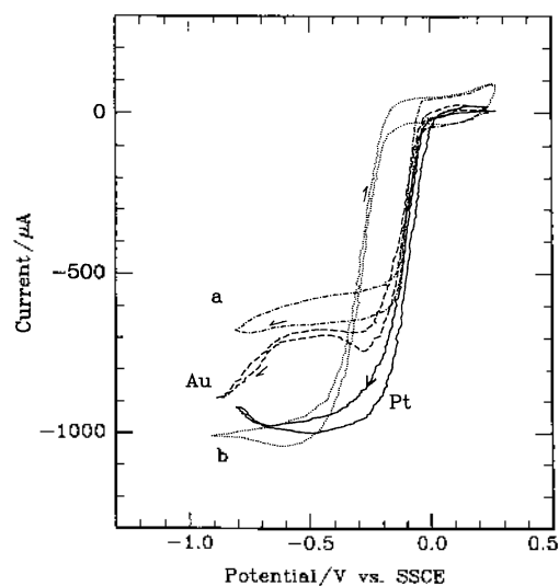
Figure 3. O 2 reduction currents at rotating PEDT-CoTSP (a), PEDT-FeTSP (b), Pt, and Au electrodes in O 2 -saturated 0.1 M KOH. Scan rate: 50 mV s -1 ; Rotation rate: 2000 rpm; Electrode area: 0.164 cm 2 .
