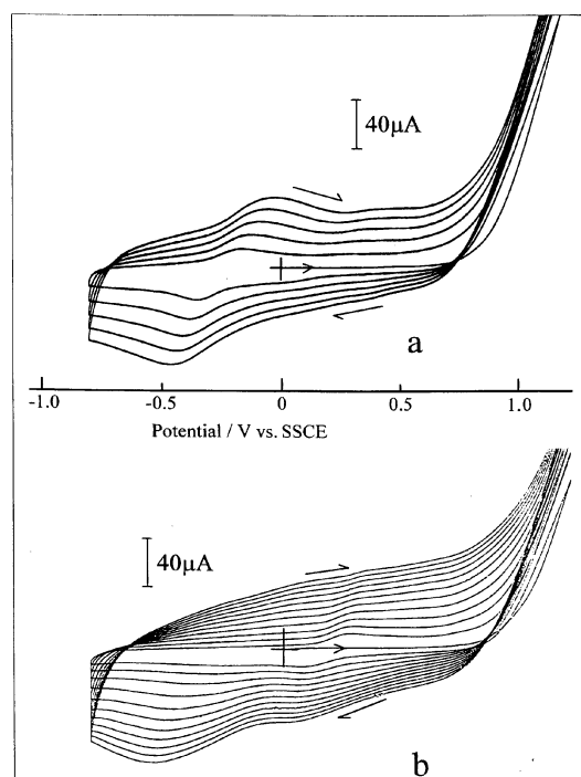
Figure 1. Electropolymerization of EDT on GC electrode with cyclically scanned potential in aqueous solution of 10 mM EDT and 1.0 mM FeTSP (a) or 1.0 mM CoTSP (b). Scan rate: 50 \text{mV s}^{-1} .
