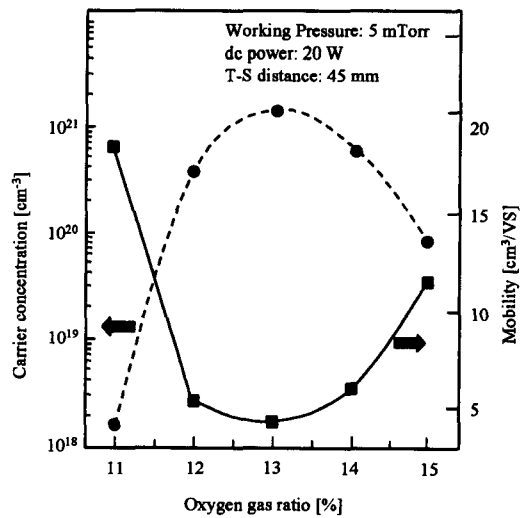
Fig. 6. Variation in carrier concentration and mobility of ITO thin films deposited as a function of O 2 partial pressure.
