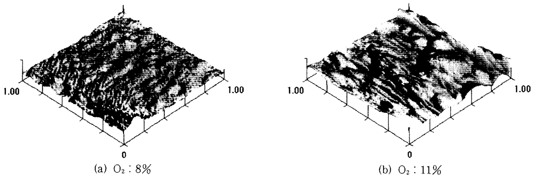
Fig. 1. AFM images of ITO films on PET substrate at different O 2 partial pressures.
