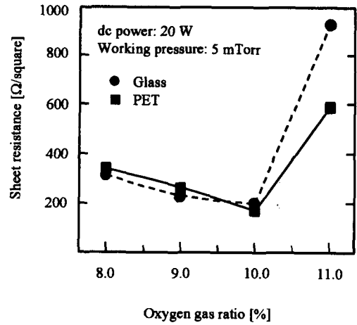
Fig. 2. Sheet resistance verse O 2 partial pressure in ITO/PET thin films.
