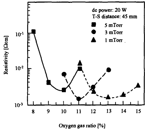
Fig. 3. Resistivity verse O 2 partial pressure with different working pressures in ITO films.
