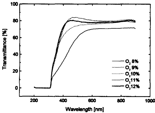
Fig. 4. Variation in transmittance of ITO films deposited as a function of O 2 partial pressure at the working pressure of 5mTorr.
