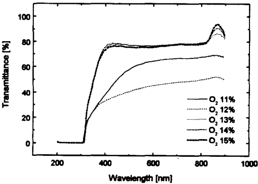
Fig. 5. Variation in transmittance of ITO films deposited as a function of O 2 partial pressure at the working pressure of 1mTorr.
