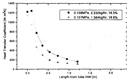
Fig. 10. Inlet Steam Flow Rate Effect on Heat Transfer Coefficient
