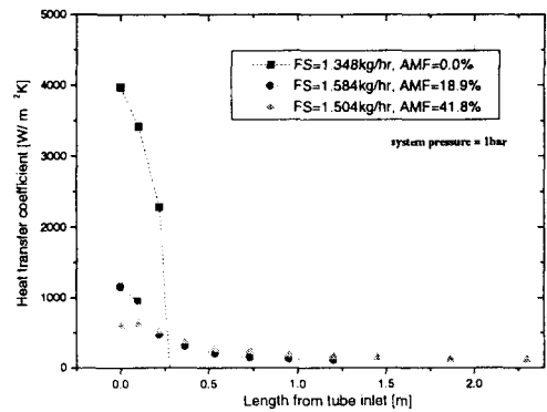
Fig. 9. Air Mass Fraction Effect on Heat Transfer Coefficient
