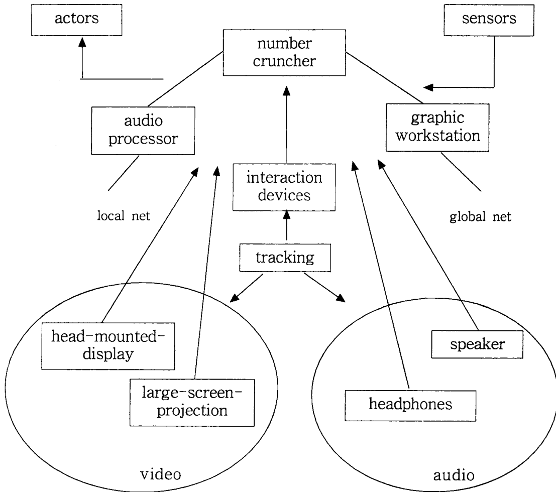
Fig. 1. Device configuration for virtual reality
